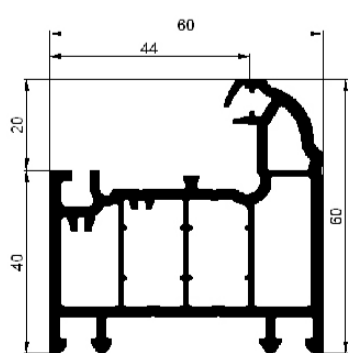
Casement 60mm Outer Frame
